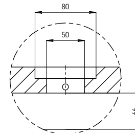
DETAIL D SCALE 1:4
